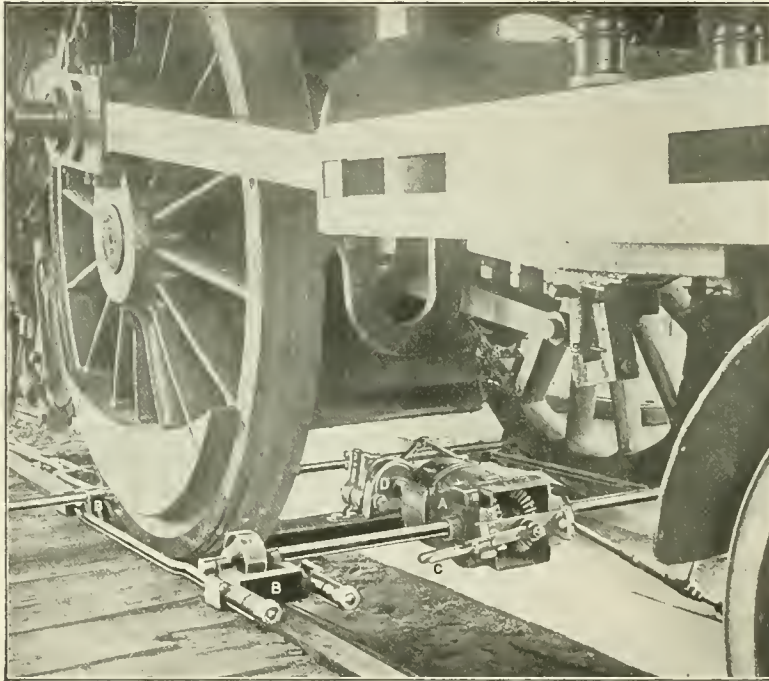
WHEEL ROTATING APPARATUS.
